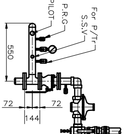
DETAIL: "B" SENSING HEADER
